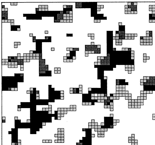
FIG. 5. A map of the distribution of first flip times \tau among the sites on a 50 \times 50 lattice at a high temperature, T^* = 1.67 . The magnitude of \tau is represented as follows: \log_{10}(\tau) < 0.8 (white), 0.8 < \log_{10}(\tau) < 1.85 [ = \log_{10}(t^*) ] (light gray), 1.85 < \log_{10}(\tau) < 2.8 (dark gray), and 2.8 < \log_{10}(\tau) (black).
