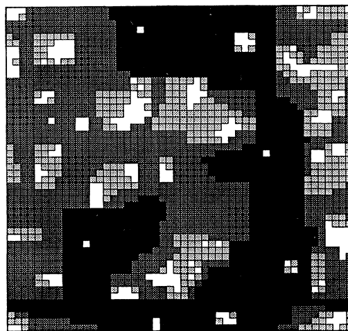
FIG. 4. A map of the distribution of first flip times \tau among the sites on a 50 \times 50 lattice at a low temperature, T^* = 0.83 . The magnitude of \tau is represented as follows: \log_{10}(\tau) < 2.0 (white), 2.0 < \log_{10}(\tau) < 3.76 [ = \log_{10}(t^*) ] (light gray), 3.76 < \log_{10}(\tau) < 6 (dark gray) and 6 < \log_{10}(\tau) (black). Note the isolated rectangles of fast spins indicating trapped pockets.
