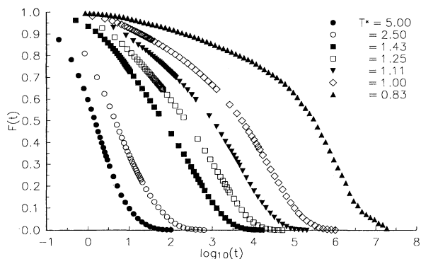
FIG. 1. The relaxation function F(t) plotted against \log_{10}(t) for 1/T^* = 0.2, 0.4, 0.7, 0.8, 0.9, 1.0, and 1.2 (corresponding to T^* = 5.00, 2.50, 1.43, 1.25, 1.11, 1.00, and 0.83, respectively).
