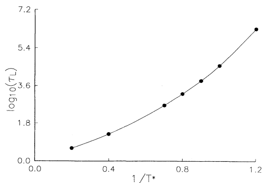
FIG. 2. \log_{10}(\tau_L) is presented as a function of 1/T^* , clearly exhibiting a non-Arrhenius temperature dependence.
