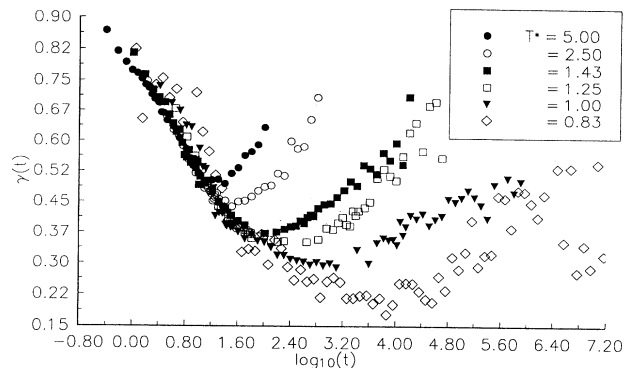
FIG. 6. The function \gamma(t) = d\{\ln[-\ln(F)]\}/d[\ln(t)] vs \log_{10}(t) for a range of T^* . A distinct minimum is observed for each temperature and its position is found to coincide with the crossover time t^* .
