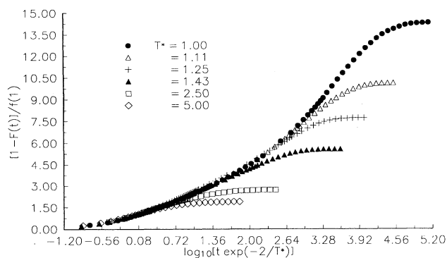
FIG. 8. A plot of the amplitude-scaled relaxation function [1-F(t)]/f(1) [with f(1) being the fraction of flippable sites] vs the scaled time t \exp(-2/T^*) . The data from different temperatures fall upon a common curve at short and intermediate times, supporting the predicted scaling described in the text.
