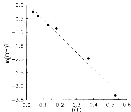
FIG. 9. The plot of the log of the relaxation amplitude \ln[F(t^*)] at the crossover time vs f(1) , the density of flippable sites, is well described by a straight line. This is in agreement with the overlap model expressed in Eq. (3). The parameter b in this equation is found to be \approx 6 .
