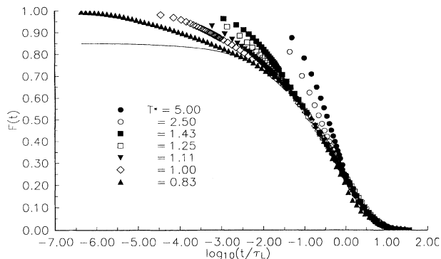
FIG. 3. The relaxation function F(t) vs \log_{10}(t/\tau_L) for the same temperature as shown in Fig. 1. Note the appearance of a common curve at long times. The solid line is a fitted stretched exponential function, 0.85 \exp[-(t/\tau_L)^{0.48}] .
