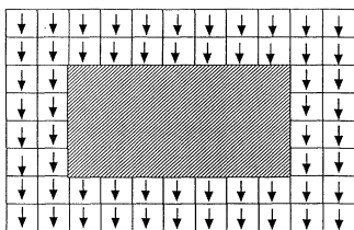
FIG. 7. An example of a “cage” in the fKI model. The enclosing wall of down spins cannot be relaxed as a result of the spin configuration within the shaded region as all the “wall” spins (with the exception of the outer corner spins) have three down neighbors and so cannot flip. The relaxation of such a region must come from outside the cage.
